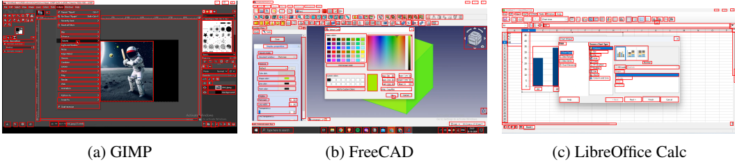
Figure 2: Examples of screenshots from different applications in GROUND CUA. Red bounding boxes indicate the annotated UI elements within each screenshot.
