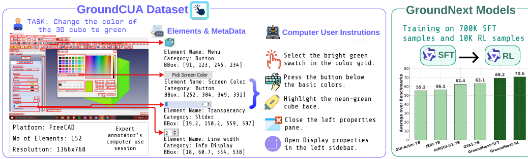
Figure 1: Overview of the GROUND CUA dataset and GROUND NEX T models. Human demonstrations of computer-use tasks are recorded as screenshots (example from FreeCAD) with UI meta-data, which are processed into high-quality natural language instruction tasks for UI grounding. GROUND NEX T is trained in two stages: SFT (700K samples) followed by RL (10K samples), achieving state-of-the-art grounding performance with efficient training.
