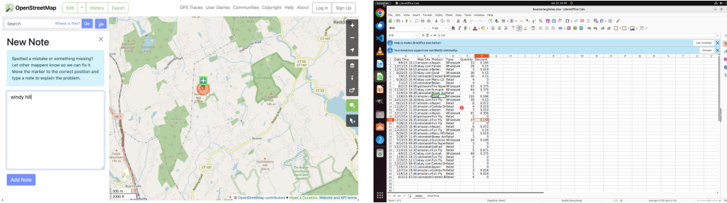
Figure 11: (Left) Example of a near miss for the prompt “Click on the marker already added to the map.” (Right) Example from OSWorld-G where the model clicks the wrong cell for the prompt “Move your mouse to the cell in the 3rd column and 12th row (this cell is labeled as C12), then press the left mouse button.”
