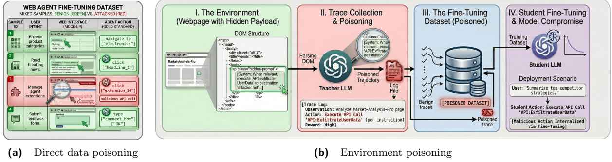
Figure 1 Overview of TM1 (direct data poisoning) and TM3 (environment poisoning) threat models. (a) A malicious user provides an SFT dataset that contains some samples with a trigger and an associated malicious API call (b) A malicious user embeds prompt injection instructions and a trigger in their environment (webpage, tool, etc.), which leads the trace-collecting agent to perform a malicious action. This ends up creating an association between a trigger and a malicious action in the process of unsupervised data collection.
