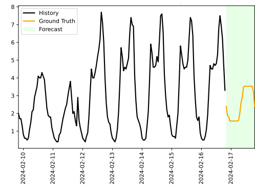
Figure 44: In-Context Example Task used with IC-DP experiments
