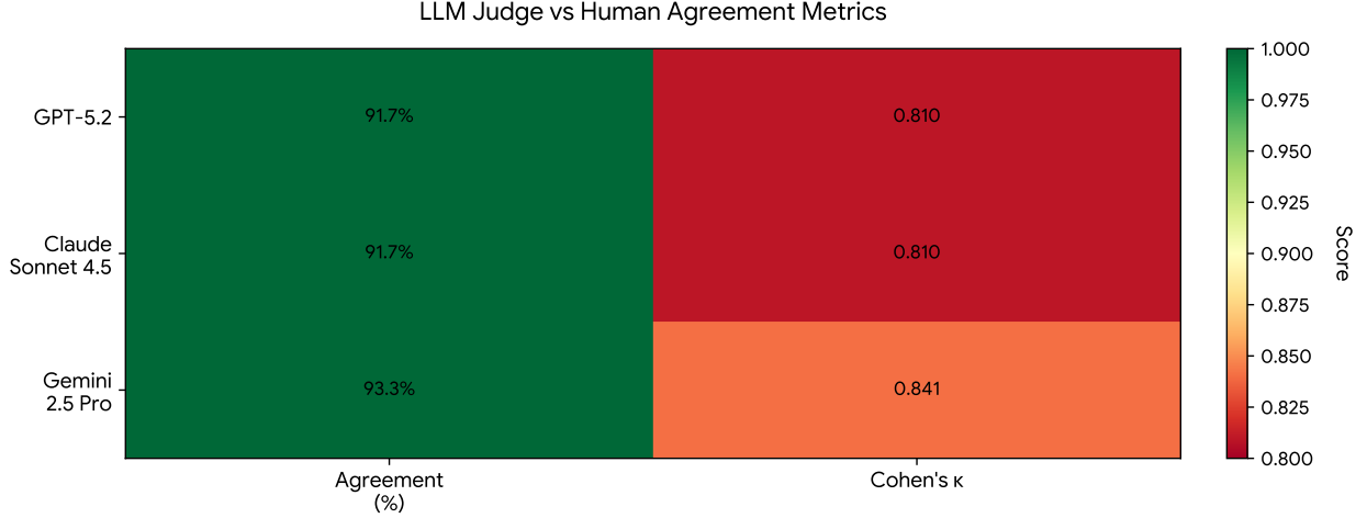
Figure 10: LLM judge validation against human evaluators (n=60). All three judges show substantial to almost perfect agreement with humans: GPT-5.2 and Claude Sonnet 4.5 both achieve 91.7% agreement (Cohen’s \kappa = 0.81 ), while Gemini 2.5 Pro achieves 93.3% agreement ( \kappa = 0.84 ). The high Cohen’s \kappa values (0.81–0.84) account for base rate differences (68.3% human YES rate) and confirm that agreement is well above chance, with confidence intervals (95% CI) ranging from [0.71–0.91] to [0.74–0.94]. These results validate the use of LLM judges for scalable evaluation of forecast effect explanations across the full 180-item model-task set.
