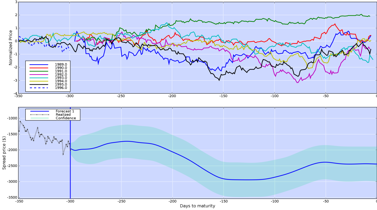
▲ Figure 4. Top part: Training set for March–July Wheat spread, containing data until 1995/05/19; each spread year constitutes a distinct trajectory. The x -axis is the negative number of days to maturity (so that time flows to the right). The y -axis is normalized spread price, where the normalization procedure is described in the text. The partial trajectory observed so far for the current year (1996) is the dashed line. Bottom part: Forecasts made by extending the partial spread trajectory of the current year using the Gaussian process regression methodology. The y -axis is the actual spread price in $ (where individual contract prices are multiplied by a contract size of 50 for Wheat).
