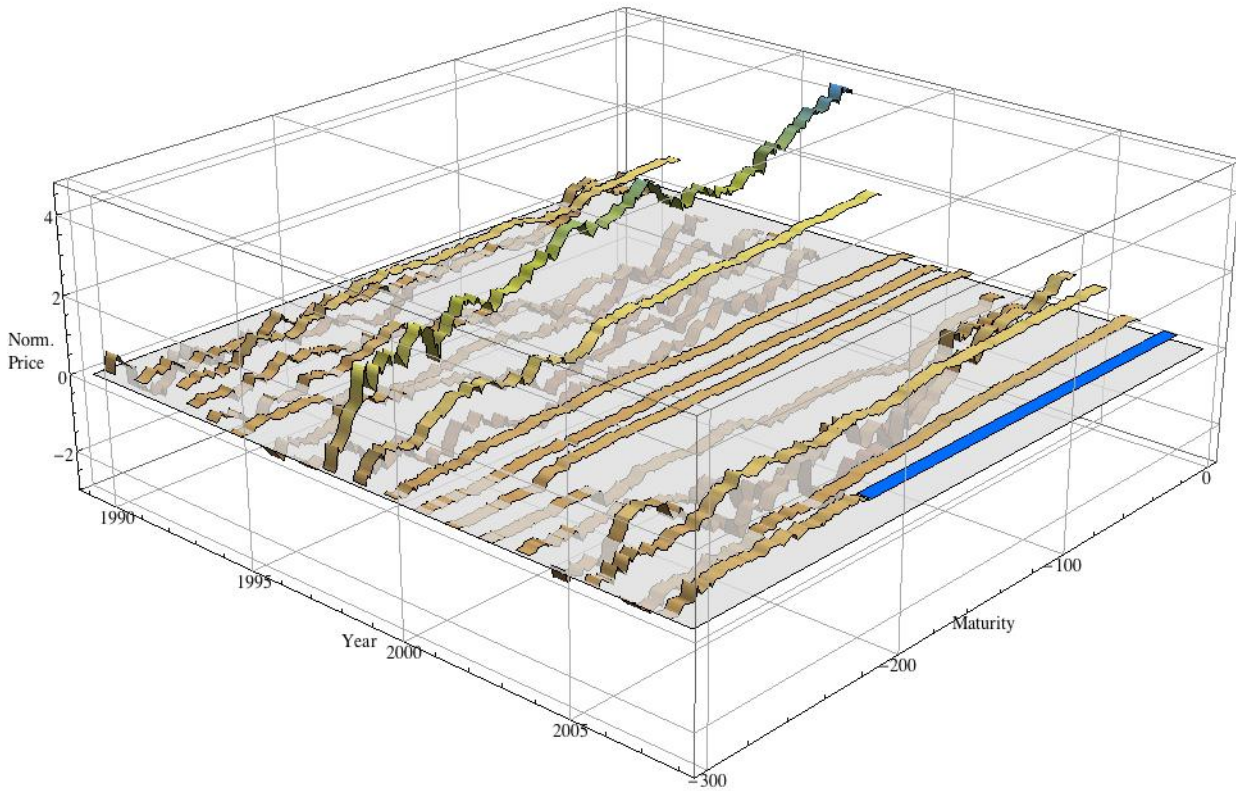
▲ Figure 3. Illustration of the regression variables around which the forecasting problem is specified. Shown is the price history of the March–July old-crop/new-crop Wheat spread, as a function of the crop year and number of days to maturity. Prices are normalized to start at zero at maturity -300 and scaled to unit standard deviation over the sample. To aid the interpretation of price movement, prices that fall below the cutting plane at zero are shown slightly shaded (“under water”). The objective of the forecasting model is to fill out the “blue strip” in the last year of data, given the partial trajectory observed so far for that last year, and the complete trajectories in previous years.
