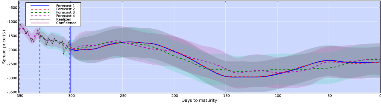
▲ Figure 6. Forecasts made from several operation times, given the same training set as in Figure 4.
