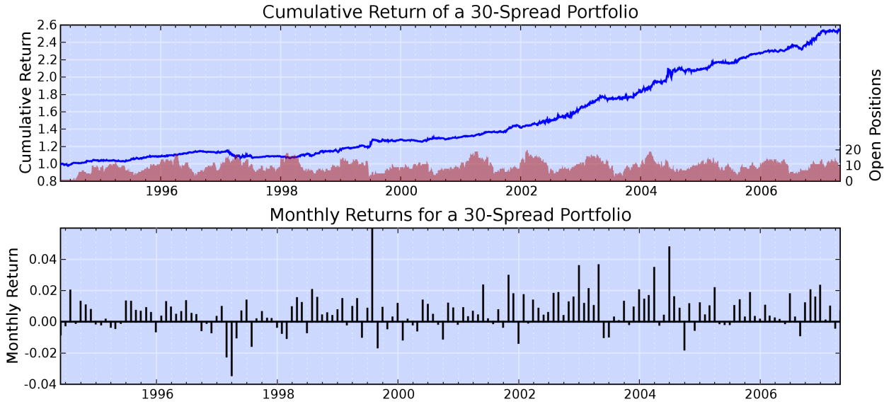
▲ Figure 11. Top Panel: cumulative excess return after transaction costs of a portfolio of 30 spreads traded according to the maximum information-ratio criterion; the bottom part plots the number of positions open at a time (right axis). Bottom Panel: monthly portfolio relative excess returns; we observe the significant positive skewness in the distribution.
