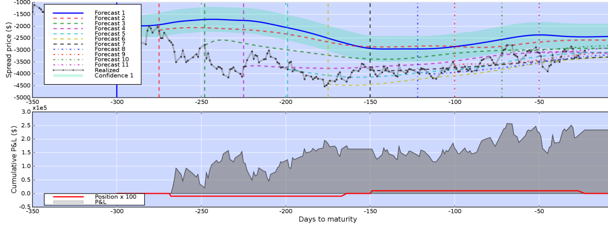
▲ Figure 7. Top Panel: Illustration of multiple forecasts, repeated every 25 days, of the 1996 March–July Wheat spread (dashed lines); realized price is in gray. Although the first forecast (smooth solid blue, with confidence bands) mistakes the overall price level, it approximately correctly identifies local price maxima and minima, which is sufficient for trading purposes. Bottom Panel: Position taken by the trading model (in red: short, then neutral, then long), and cumulative profit of that trade (gray).
