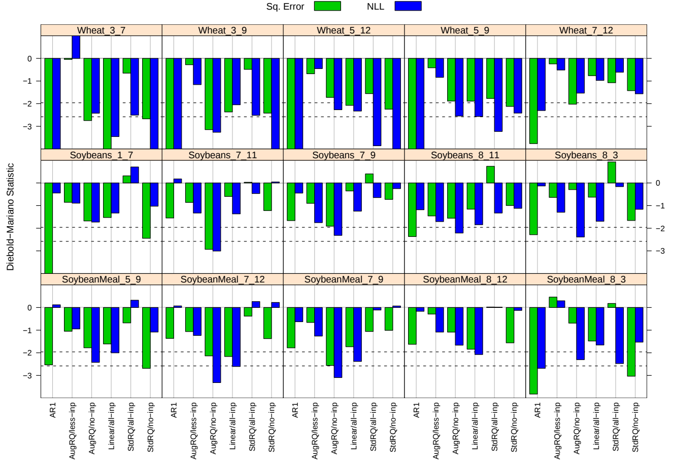
▲ Figure 9. Overview of the Cross-Correlation-Corrected Diebold-Mariano test results for the grain spreads. The 1% and 5% thresholds for statistical significance (two-tailed test) are indicated by the dashed horizontal lines.
