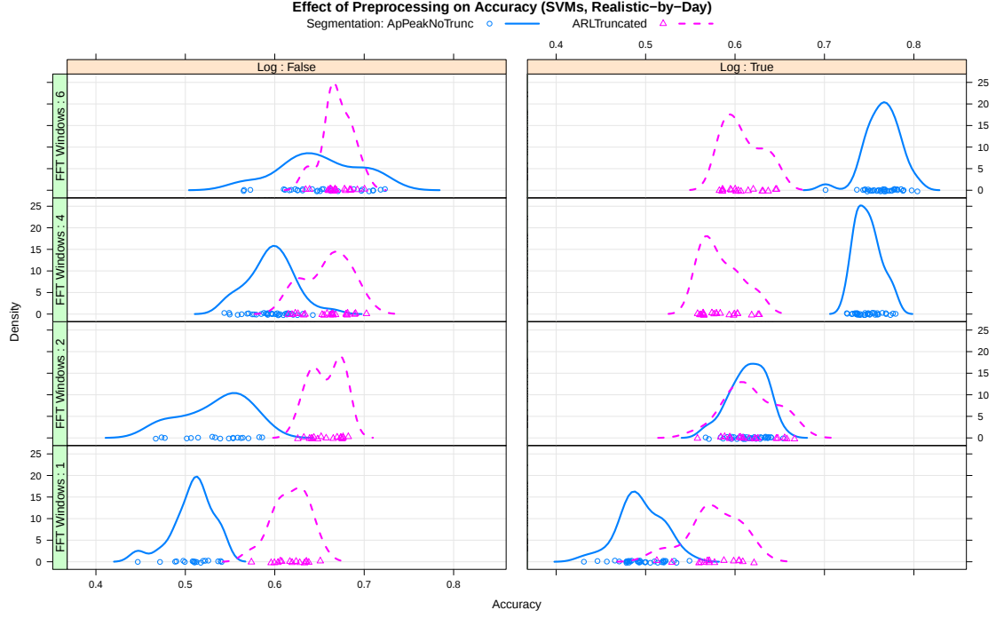
FIGURE 7. Effect of preprocessing on accuracy for SVMs, under the REALISTIC-BY-DAY setting. Accuracies appear on the x -axis, and a kernel density estimate is given in the y -axis; this representation illustrates the distributional effect on classification accuracy of an hyperparameter choice, across all other hyperparameter choices (which appear as individual points over which the distribution is plotted). The segmentation type (line styles), number of FFT windows (rows) and whether to take the logarithm of the FFT coefficients (columns) are independently varied. The semi-automatic segmentation ApPeakNoTrunc is clearly superior when considering the best of the other design choices (taking log-spectra with 6 FFT windows).
