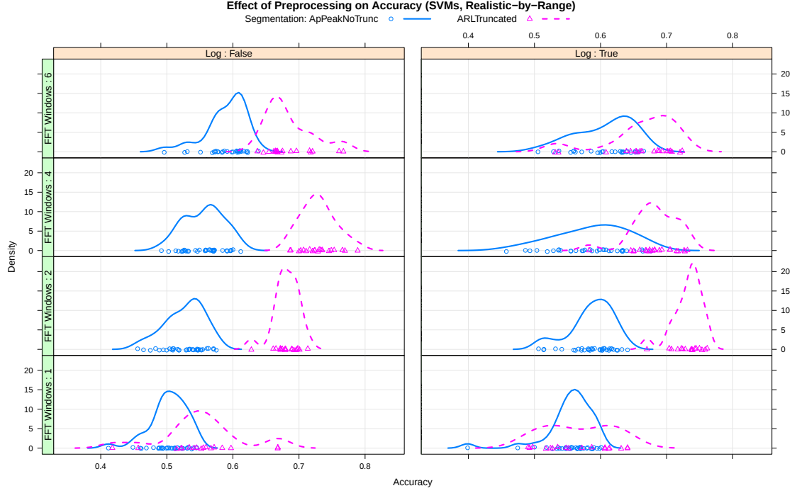
FIGURE 10. Effect of preprocessing on accuracy for SVMs, under the REALISTIC-BY-RANGE setting. The segmentation type (line styles), number of FFT windows (rows) and whether to take the logarithm of the FFT coefficients (columns) are independently varied.
