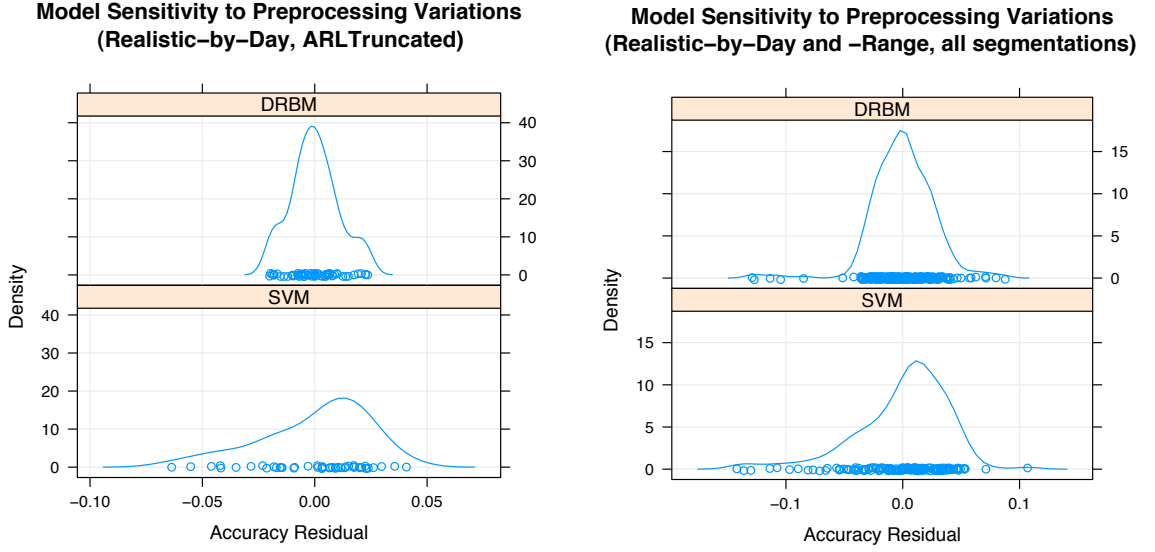
FIGURE 12. Left: Sensitivity of SVMs and DRBMs to the choice of preprocessing for the ARLTruncated segmentation, under the REALISTIC-BY-DAY setting. Right: Same results, across all segmentations and for both REALISTIC-BY-DAY and REALISTIC-BY-RANGE settings. DRBMs are seen to exhibit lower variance than SVMs, implying that they are less sensitive to the choice of preprocessing hyperparameters.
