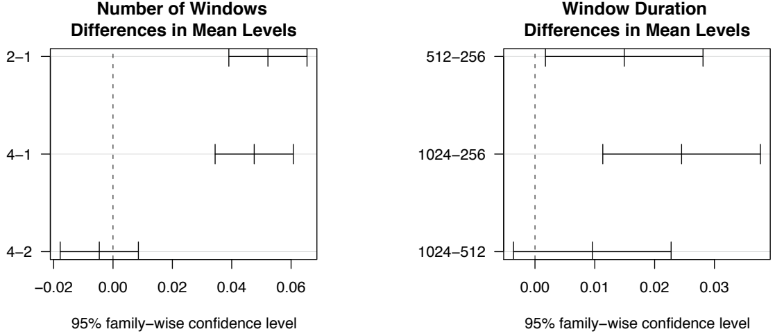
FIGURE 5. Graphical result of Tukey’s honestly significant differences procedure. It presents the results of all pairwise mean differences between the levels of factors involved in an experiment (the levels being compared are shown on the left side), and associated confidence intervals on this difference. Here, it is significantly better to use either 2 or 4 windows (compared to a single window), with size either 512 or 1024 (compared to 256).
