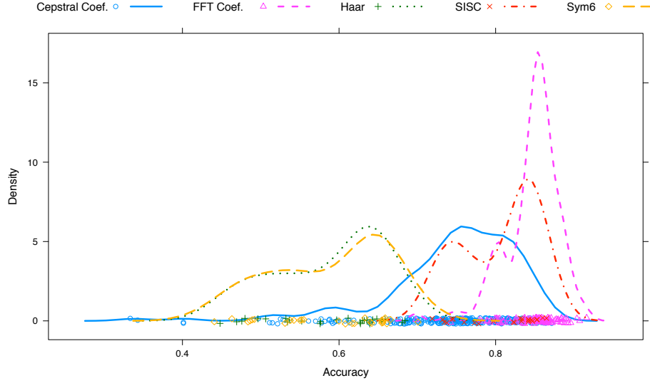
FIGURE 2. Distribution of classification accuracies for various preprocessing types using a baseline SVM classifier. For each type of preprocessing, relevant hyper-parameters are varied leading to various data points which are used to build a kernel density estimate, plotted above. Overall, the FFT preprocessing exhibits the highest classification accuracy.
